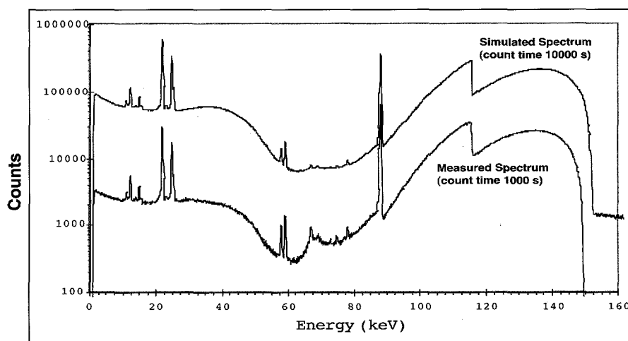
Fig. 1. Simulated densitometry spectrum of 200 g/l uranium solution and measured spectrum.
